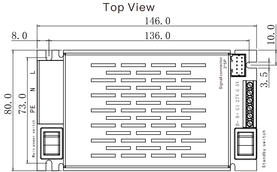
Installation size diagram, unit: mm
